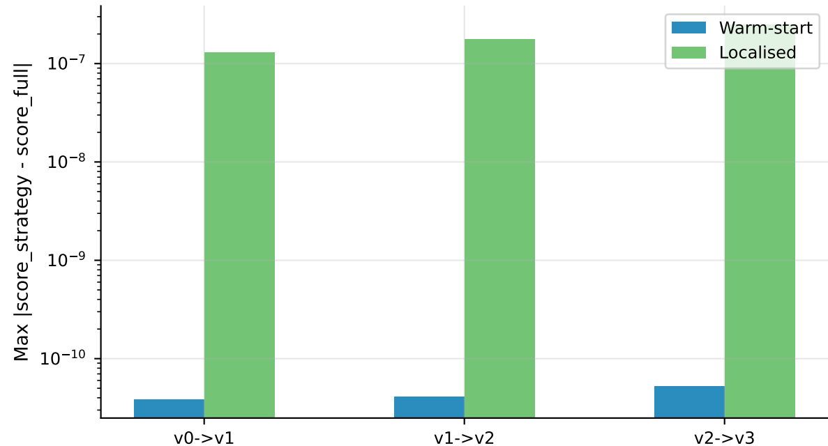
Group C - Accuracy degradation per snapshot
